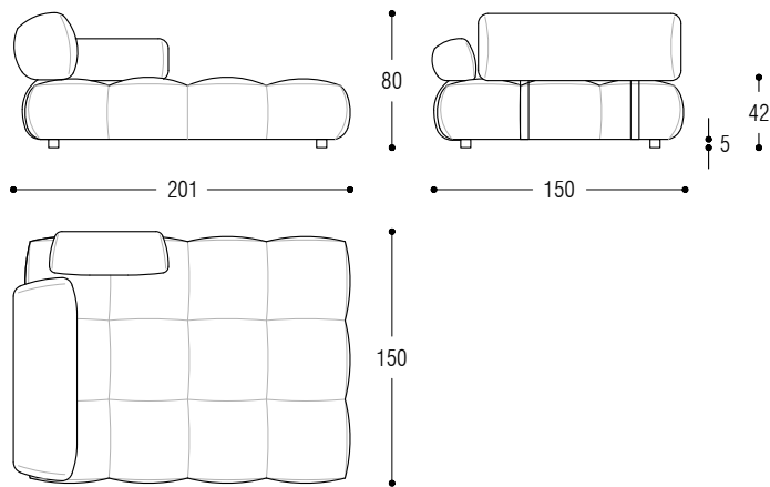
Chaise longue cm 201 WIDE with armrest right (also available left)
