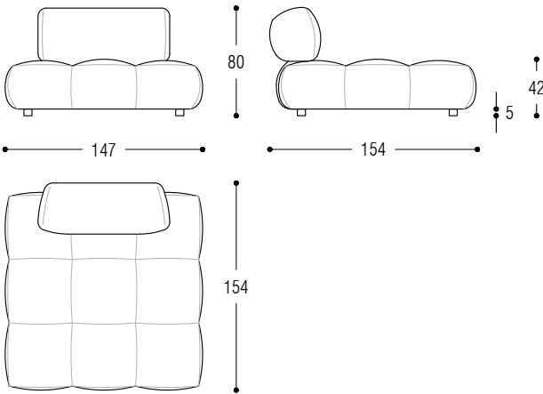
Central element cm 147 maxi
