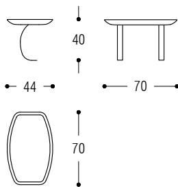
Side table cm 70x44 in black ash wood
