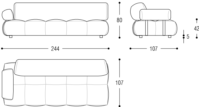
Element cm 244 WIDE left
