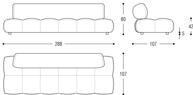
Central element cm 288
