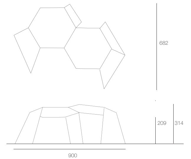
CA16D 2 hexagon tops with 4 supporting panels
