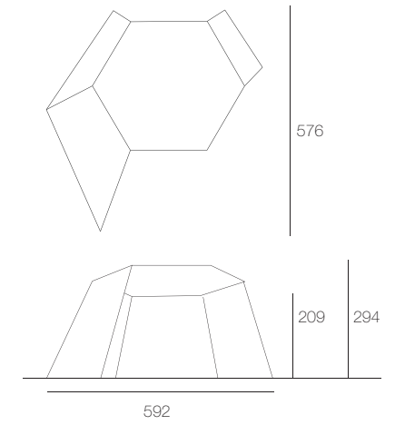
CA16D 2 hexagon tops with 4 supporting panels
