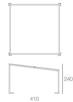
CA17G shading structure
