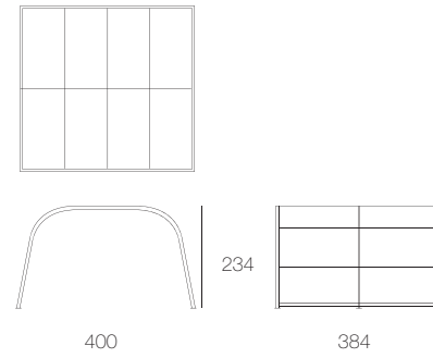
CA02ATH Modulo Tunnel in fabric without base, high uprights
