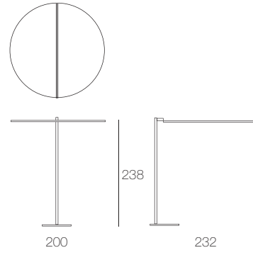
CA07B parasol with base
