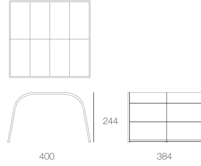
CA02ATB Modulo Tunnel in fabric with base, low uprights
