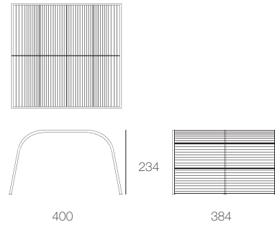
CA02AH Modulo Tunnel in wood without base, high uprights
