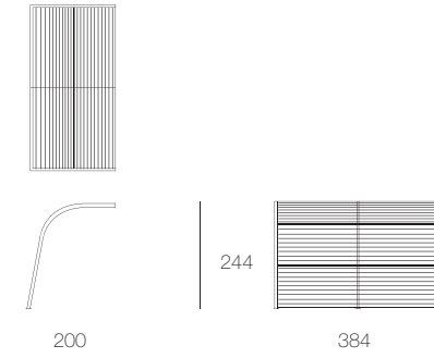
CA01FB Modulo Veranda in wood with base, low uprights
