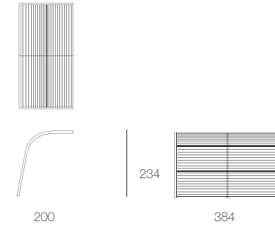
CA01FH Modulo Veranda in wood without base, high uprights
