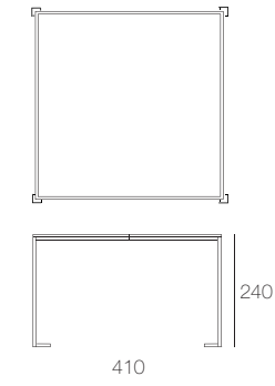
CA17B asymmetric shading structure
