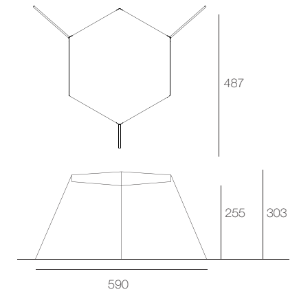
CA16A single hexagon top with 3 supporting panels
