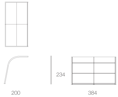
CA01FTH Modulo Veranda in fabric without base, high uprights
