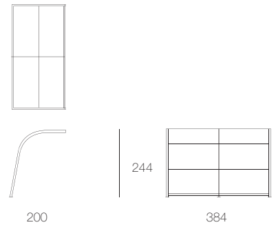
CA01FTB Modulo Veranda in fabric with base, low uprights
