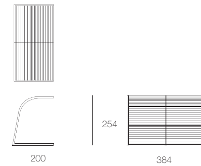
CA01FBH Modulo Veranda in wood with base, high uprights
