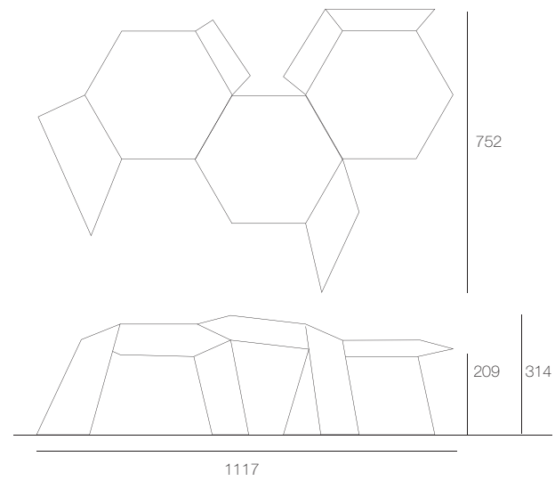
CA16B 3 hexagon tops with 5 supporting panels
