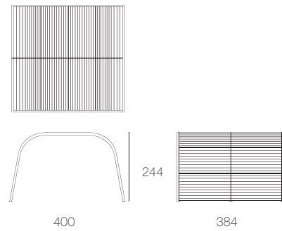
CA02AB Modulo Tunnel in wood with base, low uprights
